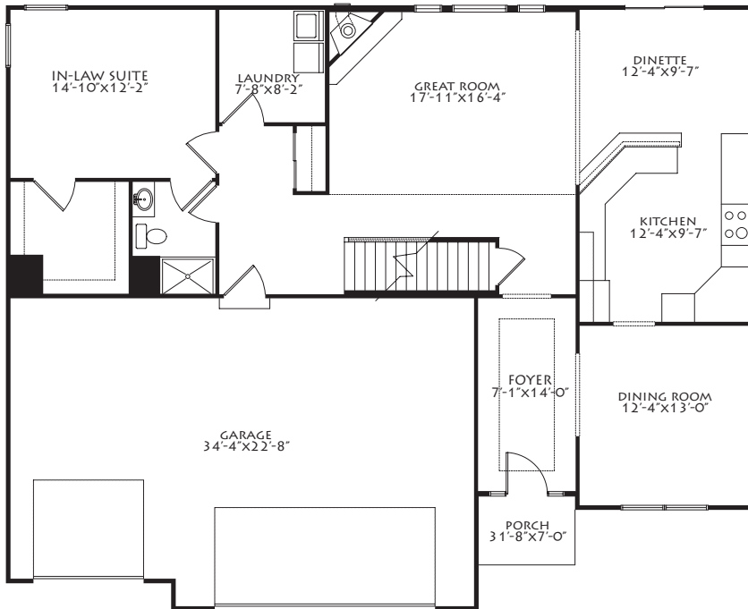
FIRST FLOOR 1462 SQFT
