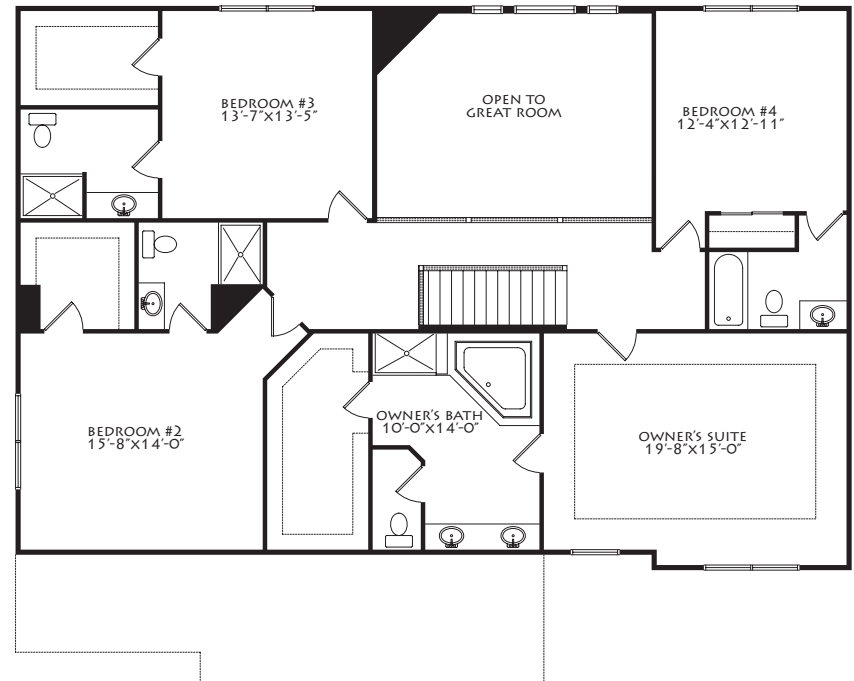
SECOND FLOOR 1655 SQFT
