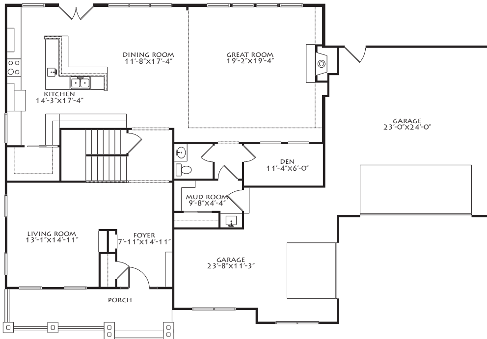
FIRST FLOOR 1640 SQFT
