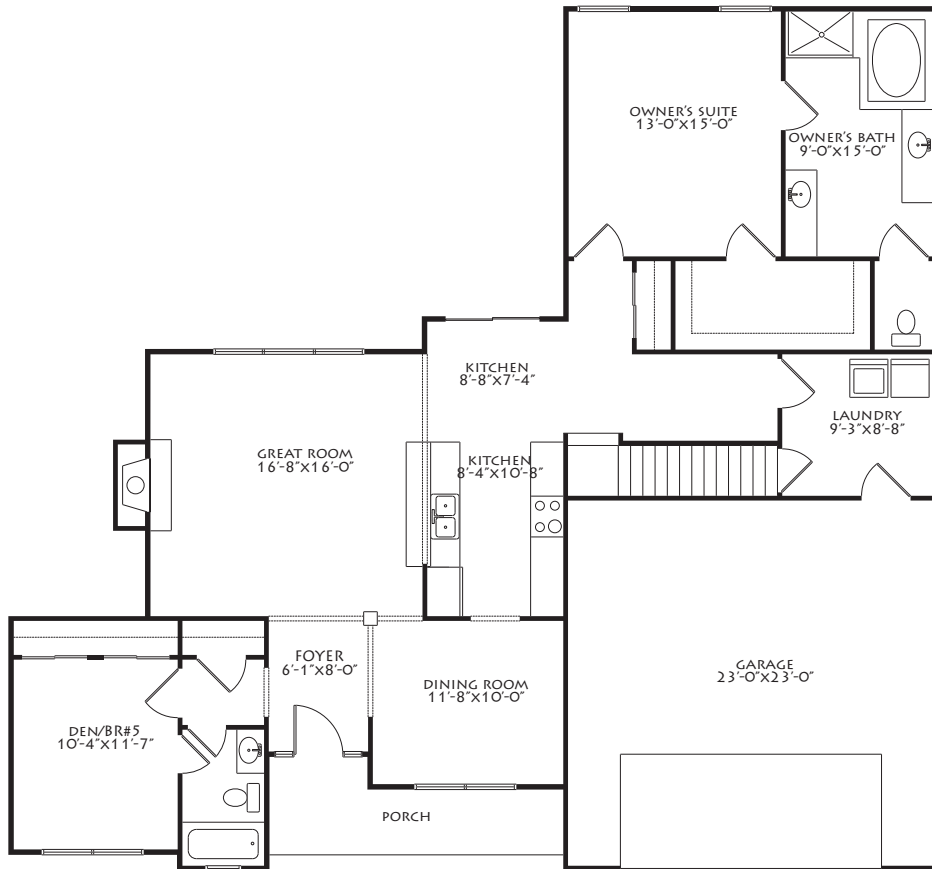
FIRST FLOOR 1569 SQFT
