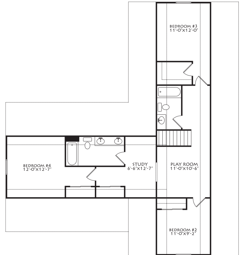
SECOND FLOOR 1002 SQFT
