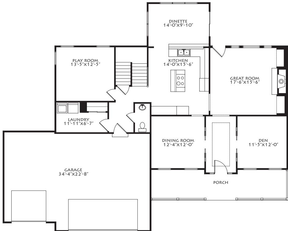
FIRST FLOOR 1518 SQFT
