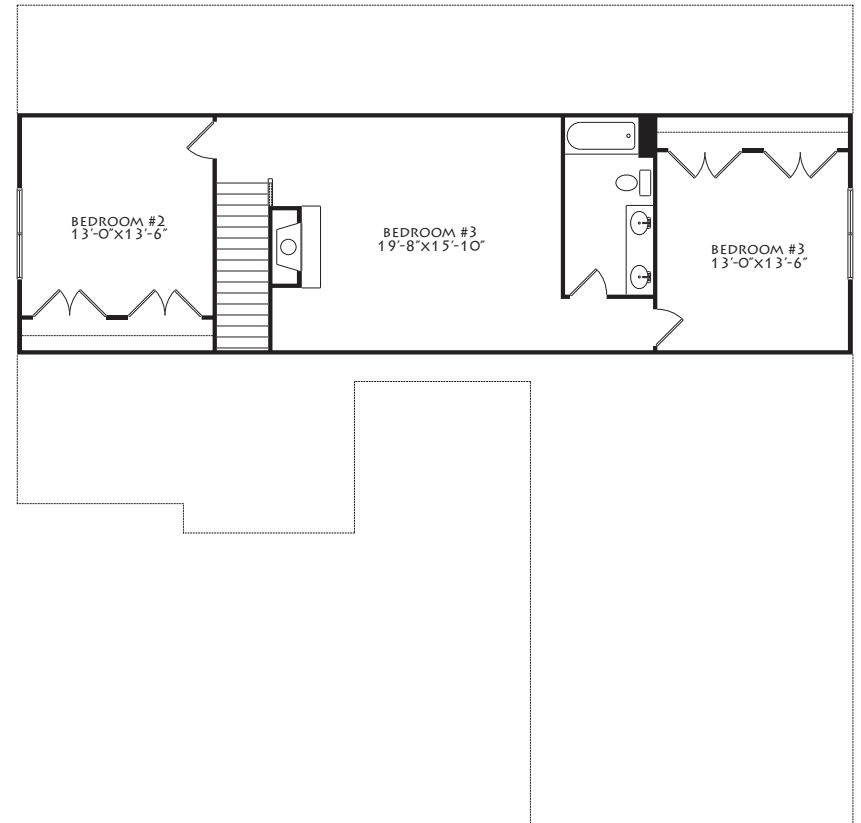
SECOND FLOOR 897 SQFT
